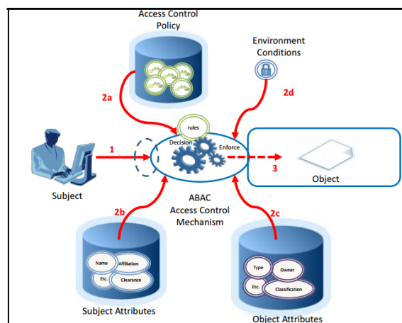
Fig. 6. Basic ABAC Scenario
