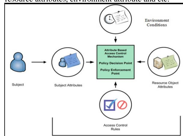
Fig. 5. Core ABAC Mechanism
