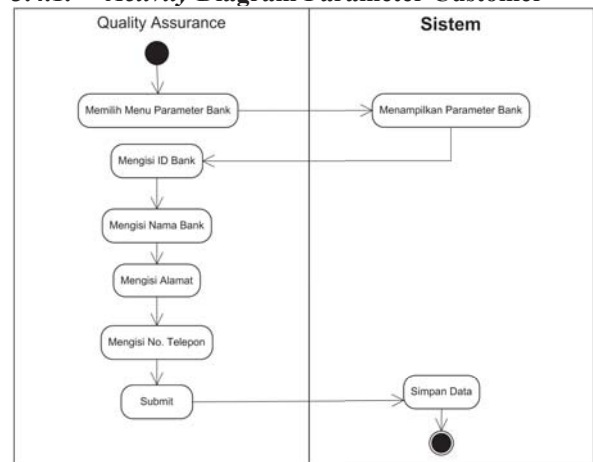
Gambar 3.3 Activity Diagram Halaman Parameter Customer
