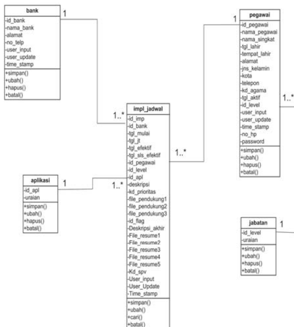
Gambar 3.5 Class Diagram
