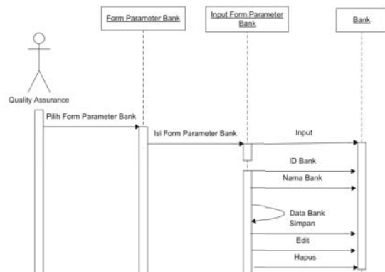
Gambar 3.4 Sequence Diagram Parameter Customer
